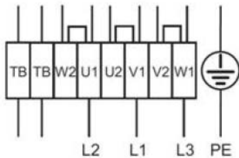
High speed \Delta -Connection
