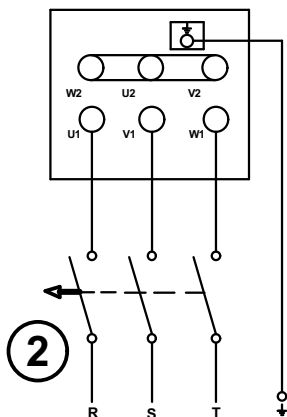
2 Interruttore magnetotermico tripolare Approvato ATEX: II (2) G/D Three phase Circuit breaker ATEX Approved: II (2) G/D
