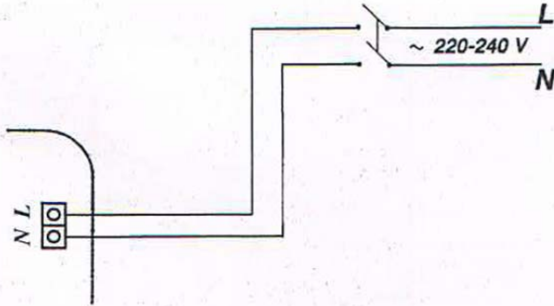
Fig. 9 COMPACT SENSOR COMPACT H (automatic)
