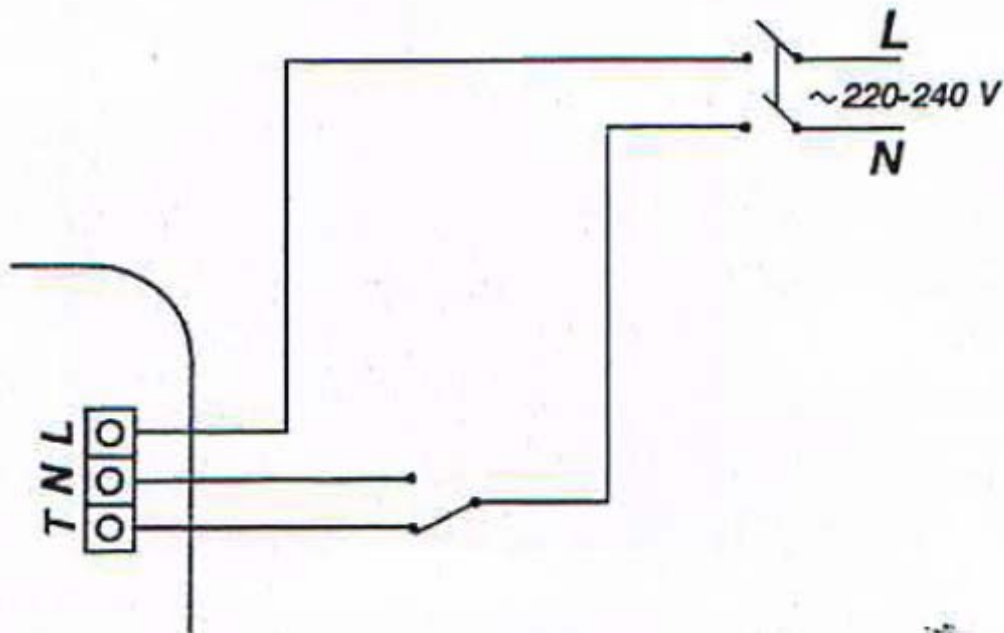
Fig. 10 COMPACT H (manual/automatic)
