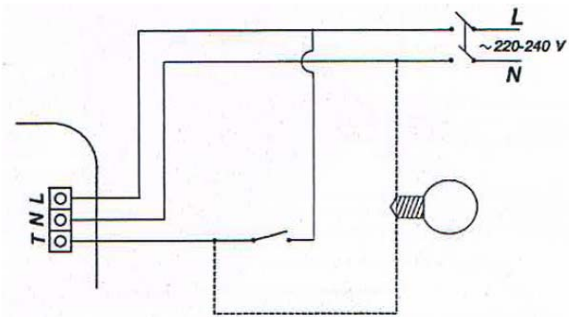
Fig. 8 COMPACT TIMER
